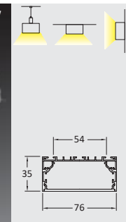
3087 Al Profile with PC Opal Matt Diffuser 1m / 4ft
