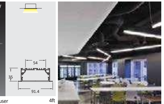
3200 Al Profile with PC Opal Matte Diffuser 4ft
