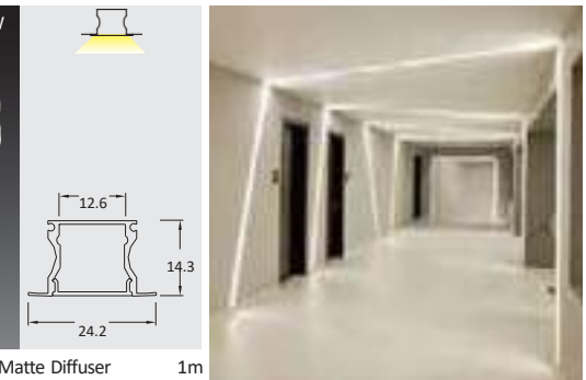
3225 Al Profile with PC Clear / Semi Clear Matte Diffuser 1m
